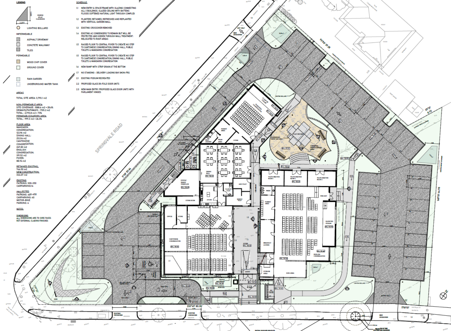
PROPOSED SITE AND GROUND FLOOR PLAN
